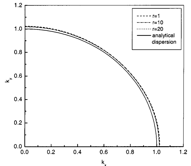
Fig. 5. Dispersion characteristics of different s at time step \Delta t = 1.5\delta_a/c ( 2.6r\times the \Delta t_{CFL} ).
